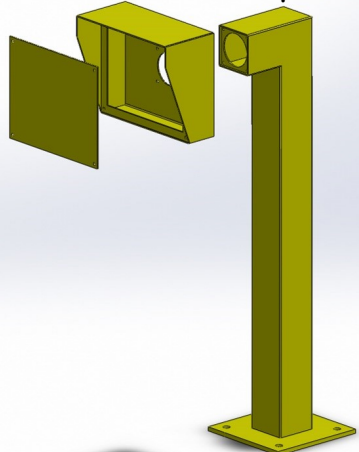
Removable reader head Removable face panel
